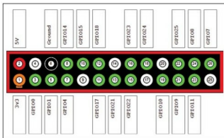
Fig. 2: Pin description of GPIO connector on Raspberry Pi
