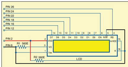
Fig. 3: Wiring diagram for connecting the GPIO of Raspberry Pi to the 16x2 LCD
