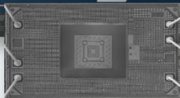
MEMS manufactured directly on top of CMOS wafer
