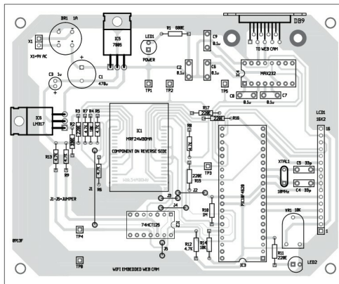
Fig. 9: Component layout for the PCB
