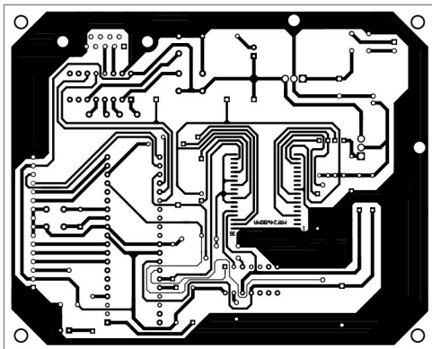
Fig. 8: Actual-size, single-side PCB layout of the Wi-Fi embedded system
