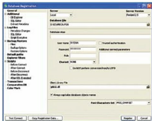
Fig. 6: IBExpert registration
