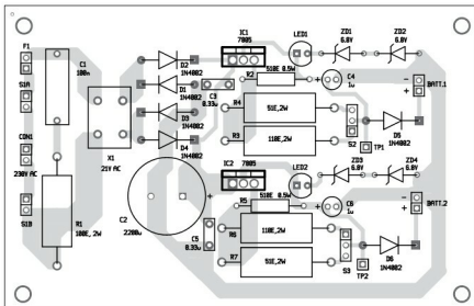
Fig. 3: Component layout of the PCB
