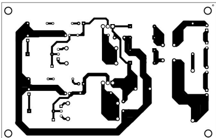
Fig. 2: Actual-size PCB of the power supply
