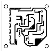
Fig. 3: Actual-size PCB of the kernel light
