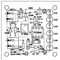
Fig. 4: Component layout of the PCB
