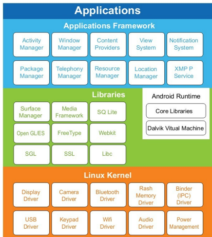
Fig. 9: Android software stack
