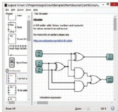
Fig. 2: A sample circuit in LogicCircuit interface
