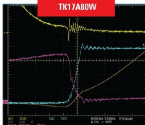
Example of turn-off Waveform VDD=400V, ID=7A, Inductive load, Rg=62Ω
