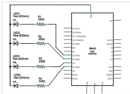
Fig. 3: Schematic diagram made using Fritzing
