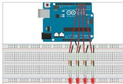
Fig. 1: Assembled circuit on a breadboard interfaced with Arduino board
