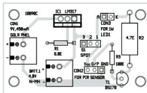
Fig. 5: Component layout of the PCB
