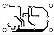
Fig. 4: Actual-size PCB of the solar light for a portable toilet
