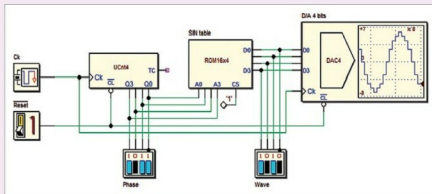
Fig. 4: A digital system with the new DAC component
