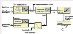
Fig. 5: Microcomputer based digital signal generator
