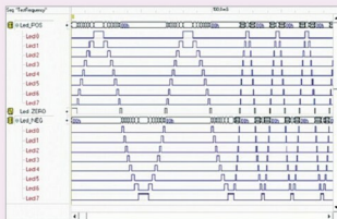
Fig. 6: Timing simulation of a signal generator
