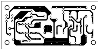
Fig. 3: Actual-size PCB of the metal detector
