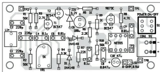
Fig. 4: Component layout of the PCB
