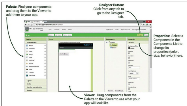
Fig. 2: App Inventor Designer
