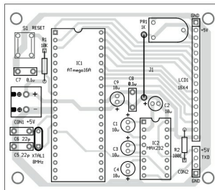
Fig. 5: Component layout of the PCB
