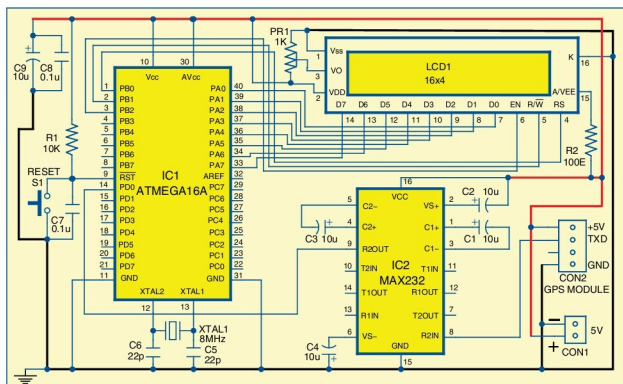
Fig. 3: Circuit diagram of the GPS receiver
