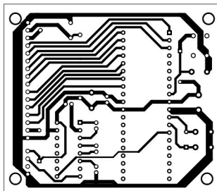
Fig. 4: Actual-size PCB pattern of the GPS receiver
