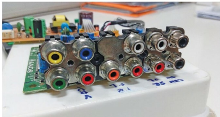
Fig. 3: AV controller board, composite component video, digital video-out; stereo cum 5.1-channel audio-out RCA connectors
