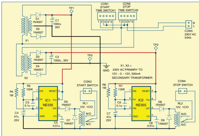
Fig. 2: Circuit diagram of the programmable on and off controller for a 3-phase electric motor
