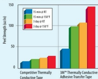
90° Peel Adhesion to Bare Untreated Aluminum
