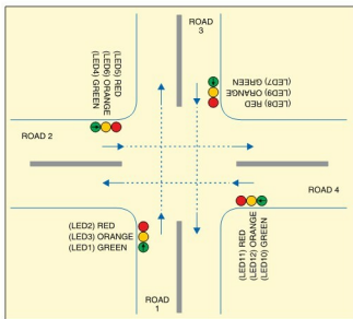
Fig. 2: Typical traffic light system on the road crossing
