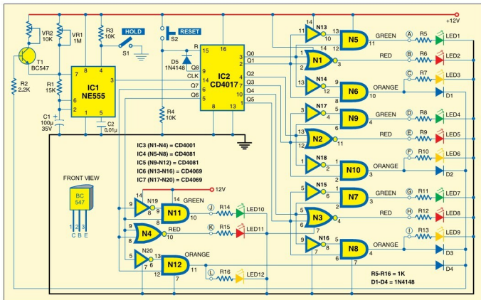
Fig. 1: Circuit of simple traffic light system
