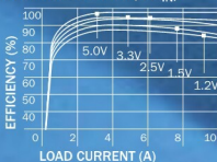
EFFICIENCY vs LOAD (12VIN)
