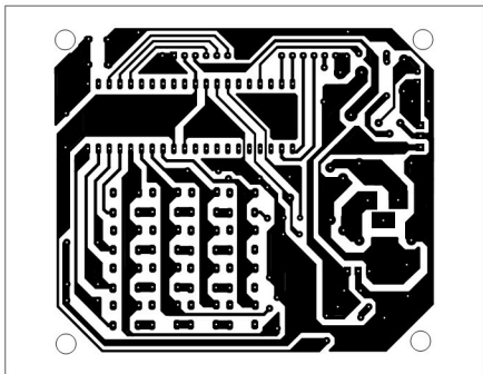
Fig. 4: Actual-size, single-side PCB for the PIC microcontroller-based electronic lock
