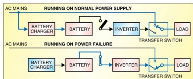
Fig. 1: Block diagram of an offline UPS
