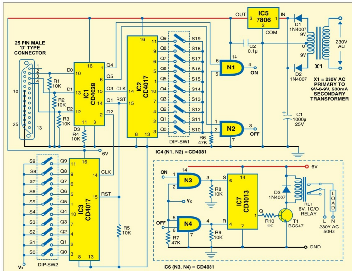
Fig. 1: Circuit of computerised electronic lock
