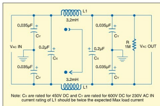
Fig. 4: A typical EMI filter
