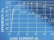
EFFICIENCY vs LOAD (12VIN)
