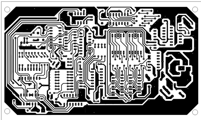
Fig. 5: Actual-size, single-side PCB for the analogue clock with add-on calendar
