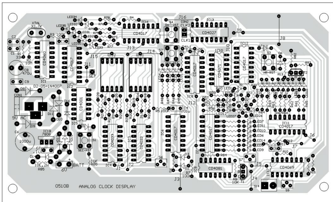
Fig. 6: Component layout for the PCB shown in Fig. 5
