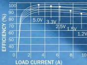
EFFICIENCY vs LOAD (12VIN)
