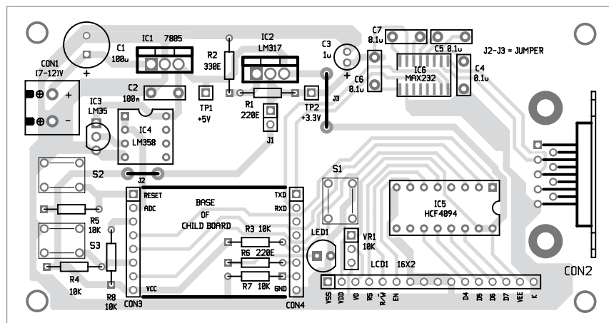
Fig. 9: Component layout of the main board
