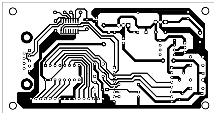
Fig. 8: Actual-size PCB pattern of the main board
