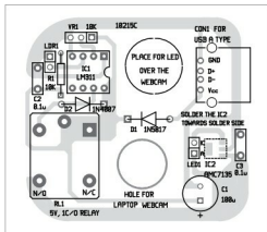
Fig. 4: Component layout of the PCB
