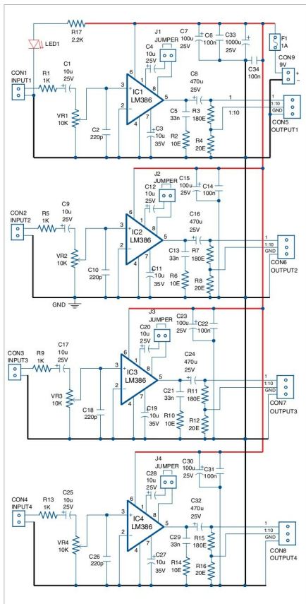
Fig. 1: Circuit of the low-cost quadraphonic amplifier
