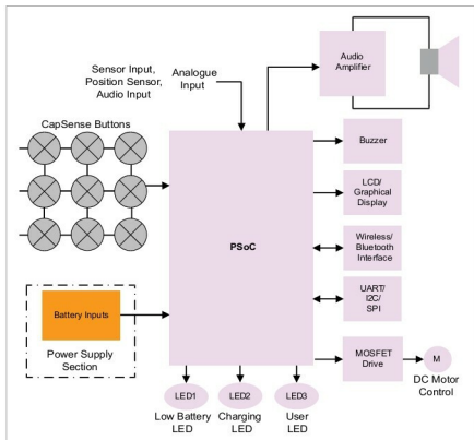
Fig. 2: PSoC based block diagram
