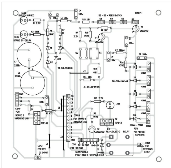
Fig. 3: Component layout of the PCB
