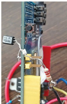
Fig. 4: Author's prototype showing transistor T3 connected to power key terminal of the GSM module
