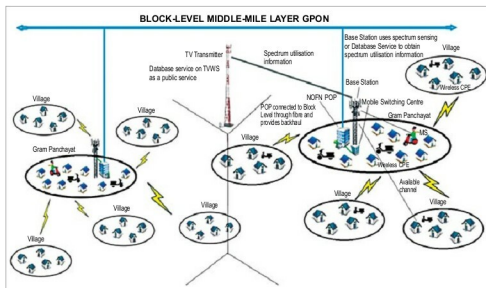
Proposed model to provide last-mile connectivity to villages using CRN based on TVWS
