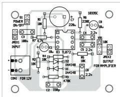
Fig. 3: Component layout of the PCB
