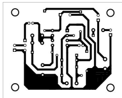
Fig. 2: Actual-size PCB pattern of the audio noise limiter
