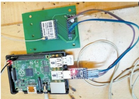
Fig. 3: GPRS shield and dongle connections
