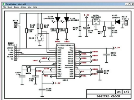
Fig. 3: A schematic drawn using CometCAD
