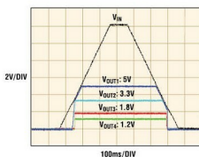
LT8602 Dropout Performance
