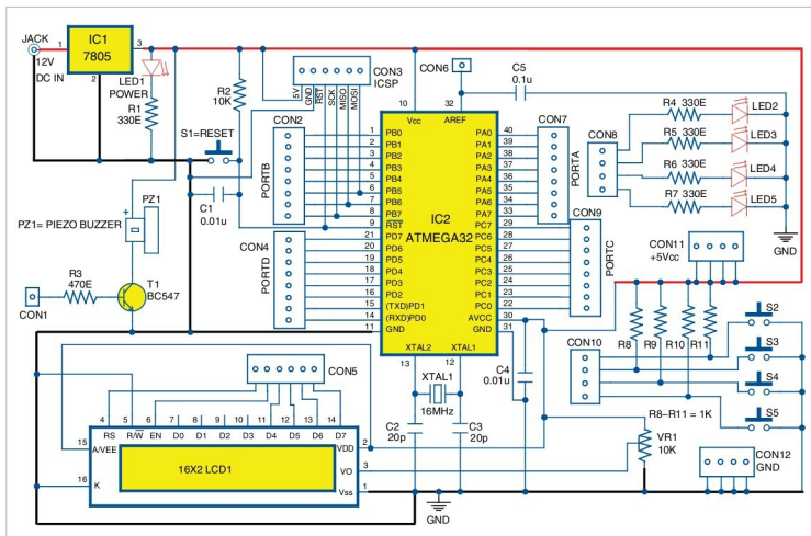
Fig. 3: Circuit diagram of Arduino for ATmega32
