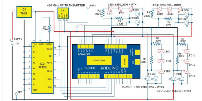
Fig. 3: Transmitter circuit of the wireless robotic car
