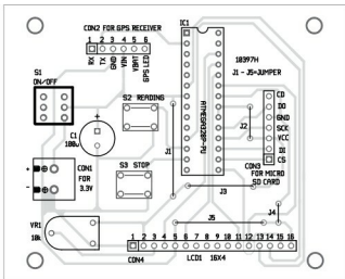
Fig. 3: Component layout for the PCB
