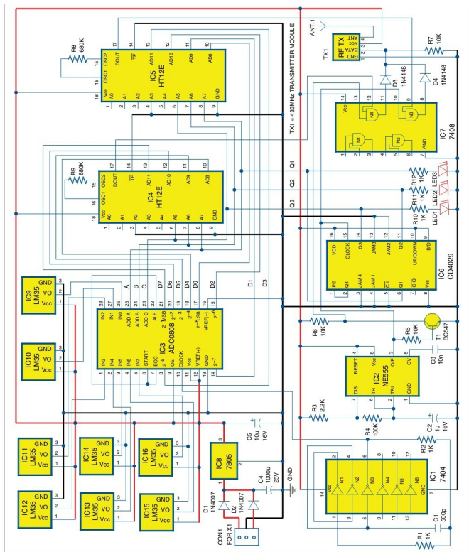
Fig. 2: Circuit diagram of the transmitter unit
