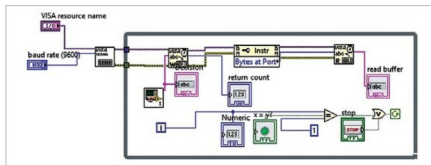
Fig. 5: Serial communication VI
