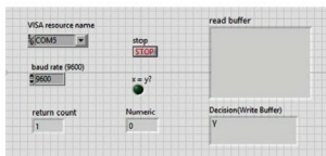
Fig. 6: Front panel of serial communication VI
