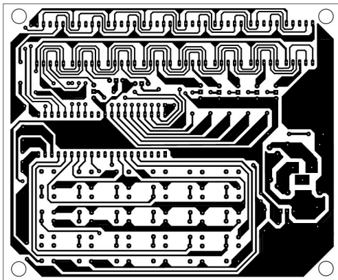
Fig. 2: An actual-size, single-side PCB for the electronic calculator
