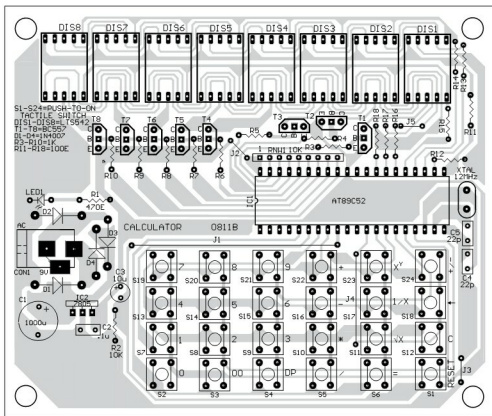
Fig. 3: Component layout for the PCB
