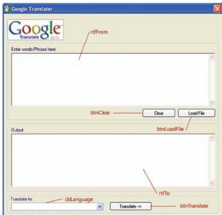
Fig. 1: FormMain after adding all required controls
