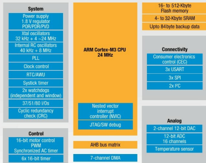
STM32 Value line block diagram
