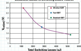
Conduction Losses vs Switching Losses Tradeoff
