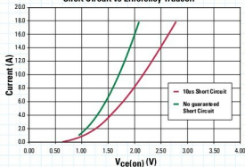
Short Circuit vs Efficiency Tradeoff
