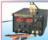
MAX 525 BATTERY ANALYZER (MOBILE TESTER) • Battery Analyzer, Micro Soldering Iron • Digital Power Supply with reconditioning system • Voltage & Ampere check with continuity buzzer • Turn ON any mobile without battery • Charge your mobile battery without mobile handset • Speaker, ringer & vibrator check
