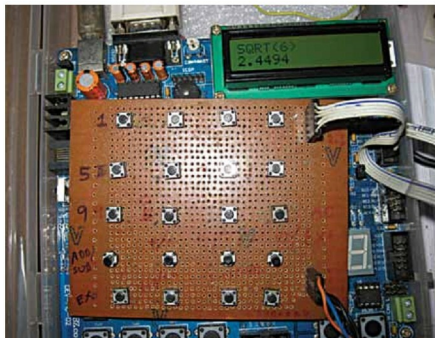
Fig. 10: Working prototype of scientific calculator
