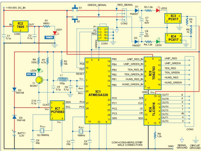
Fig. 1: Circuit of AVR-based traffic light count-down timer
