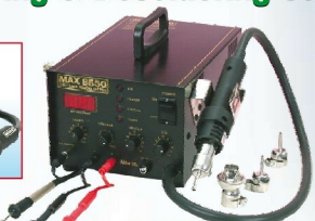
MAX 8550 SMD REWORK STATION THREE IN ONE
